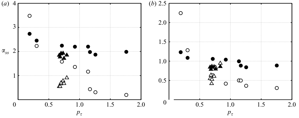
FIGURE 7. Self-similarity parameter \alpha_{ss} for numerical solutions for duration-limited case. Circles, artificial pumping; triangles, conventional parameterizations of wave input at different wind speeds. (a) Mean frequency \omega_m is used as a characteristic frequency in (1.9), (b) peak frequency \omega_p scaling. Filled symbols correspond to estimates (3.6), open symbols to (3.4).
