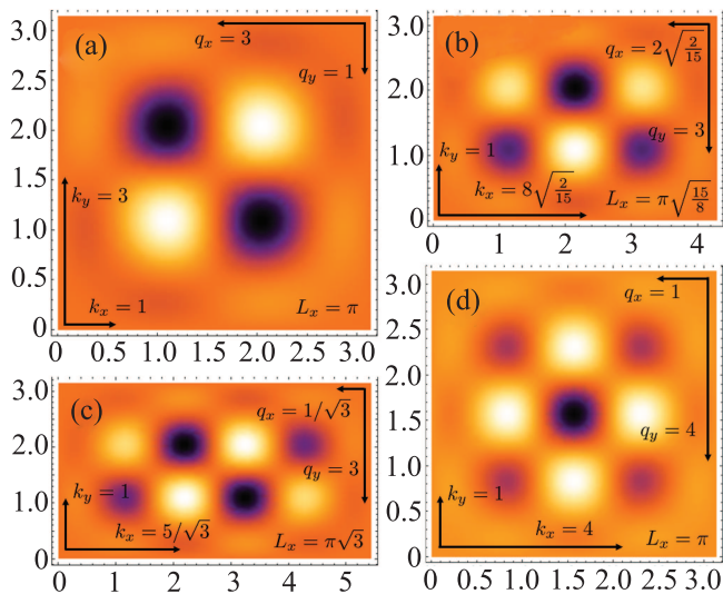
Fig. 1. (Color online) The spatial distribution of the steady vorticity \varpi_z for two standing waves (18). For all cases the second dimension of the frame L_y = \pi . The other parameters are shown in the figure
